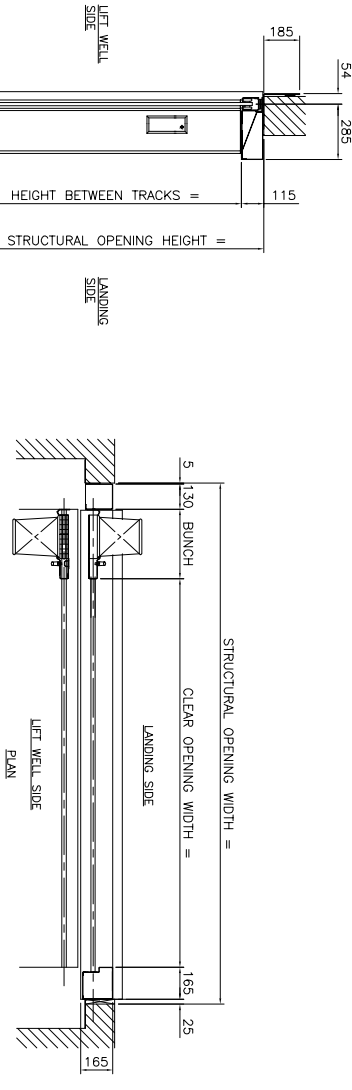
RH LANDING SHUTTER c/w 229mm LEAVES & 4 SIDED SUBFRAME ASSEMBLY
