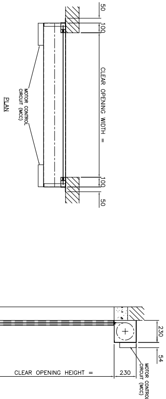
RANGE 4 – FF
